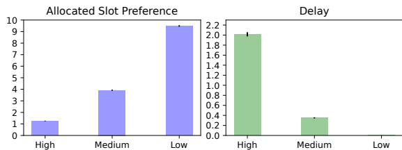
Figure 2: Priority and delay trade-off of VCG-T.
