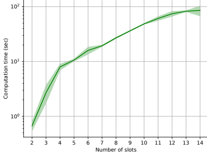
Figure 5: Computation times of VCG-T.
